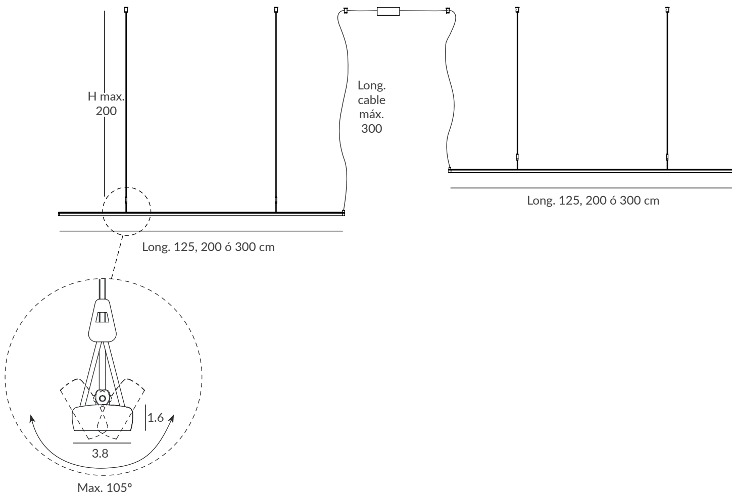
Base KIT 1 (para perfil individual) Base KIT 1 (for single profile)
